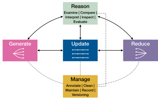
Fig. 3. The five high-level processes around alternatives: Generate, Update, and Reduce are distinguished by their different "shapes" within the alternative space (divergent, parallel, convergent). Reason and Manage do not directly produce alternatives, but operate on them.
