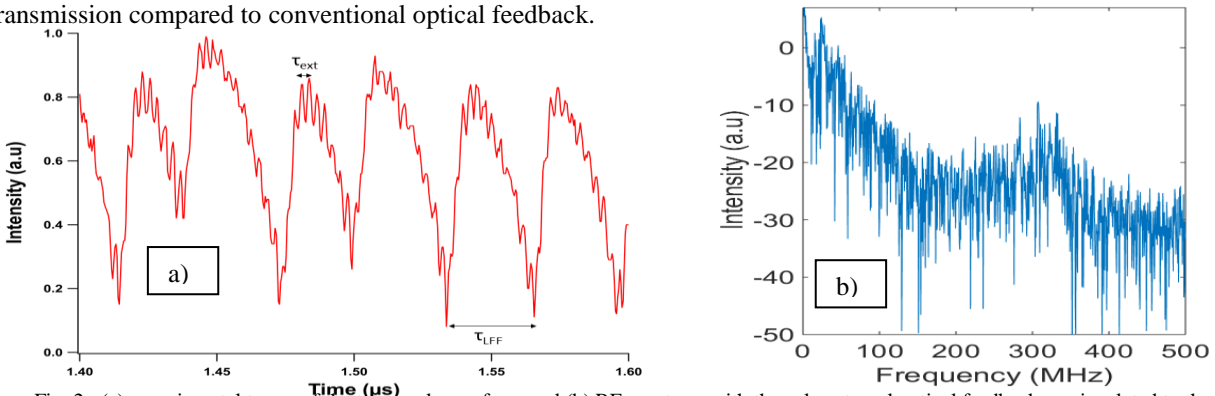
Fig. 2 : (a) experimental traces of the temporal waveform and (b) RF spectrum with the sole external feedback. \tau_{\text{ext}} is related to the frequency of the external cavity and \tau_{\text{LFF}} is related to that of LFF. Note the different timescale when comparing Fig. 2 (a) and Fig. 3 (b).
