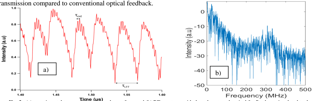
Fig. 2 : (a) experimental traces of the temporal waveform and (b) RF spectrum with the sole external optical feedback. \tau_{\text{ext}} is related to the frequency of the external cavity and \tau_{\text{LFF}} is related to that of LFF. Note the different timescale when comparing Fig. 2 (a) and Fig. 3 (b).
