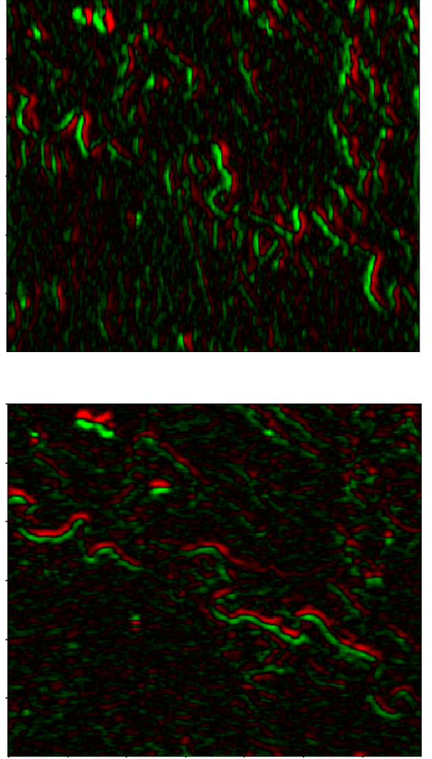
Fig. 7. Gradient for the simulated SWOT image. The positive values are displayed in green, the negative values are displayed in red. Above: horizontal gradient, below: vertical gradient. The gradients have been computed with the GR approach with a weighting parameter \alpha = 2.4 which is a good compromise between smoothing and location for L = 4 .
